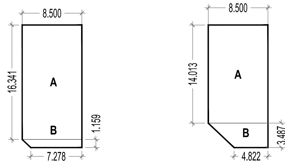
D2 PLOT AREA DETAIL
